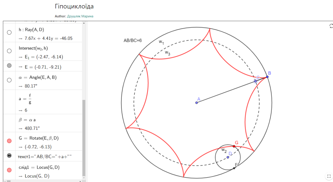
Figure 6: The hypocycloid consists of \frac{R}{r} = 6 of identical arcs.
