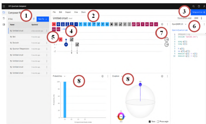
Рис. 5. IBM Quantum Composer
