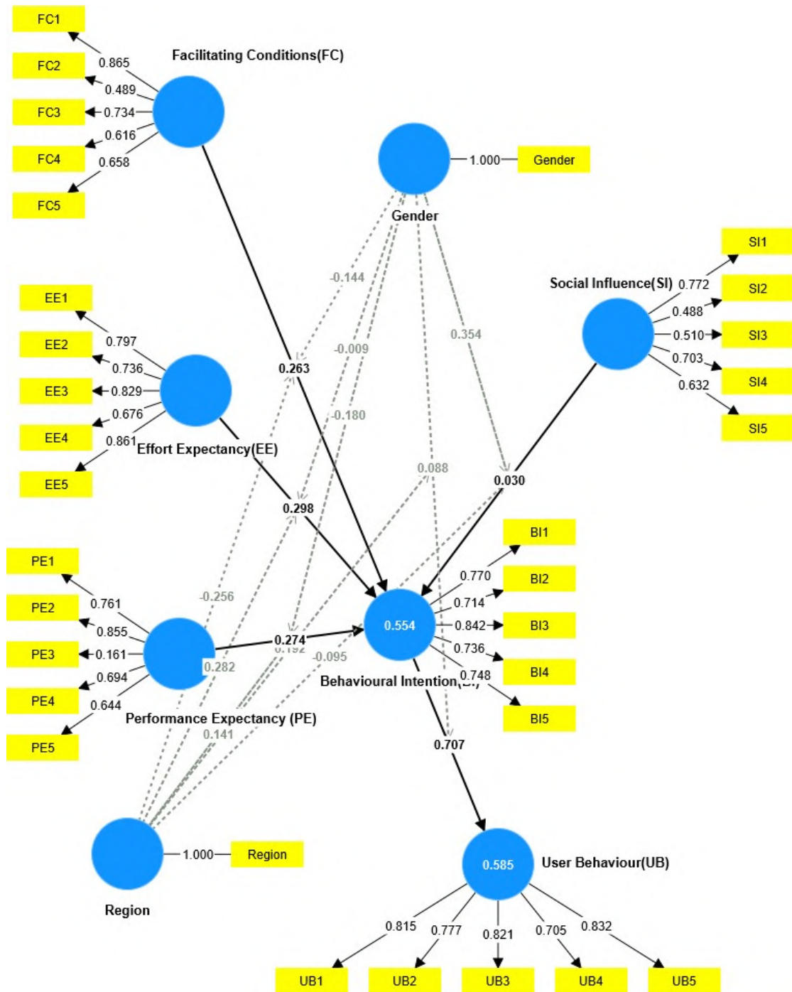
Figure 5: Confirmatory factor analysis (modified UTAUT based on figure 1).
